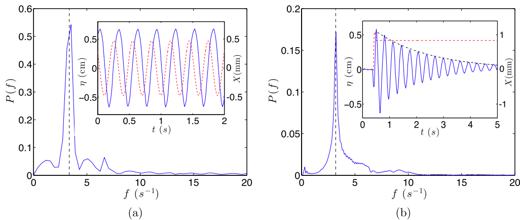
FIG. 2. Temporal spectrum P(f) of the free surface displacement measured 1 cm away from the edge of the cell for (a) a continuous sinusoidal forcing at frequency f = 3.3 Hz and (b) an impulse excitation. The vertical dashed line shows the first resonant frequency f_1 \approx 3.2 Hz. Insets: The corresponding time evolution of the free surface \eta is represented by a blue continuous line (scale: left axis). The red dotted line shows the motion of the container X(t) (scale: right axis). The black dashed-dotted line in the inset of (b) corresponds to an exponential damping, \eta_0 \exp(-t/\tau_\ell) , where \eta_0 and 1/\tau_\ell are fitting parameters. Experiments are performed with a depth H = 4 cm of foaming solution in a container of width w = 1.59 cm and length L = 7 cm.
