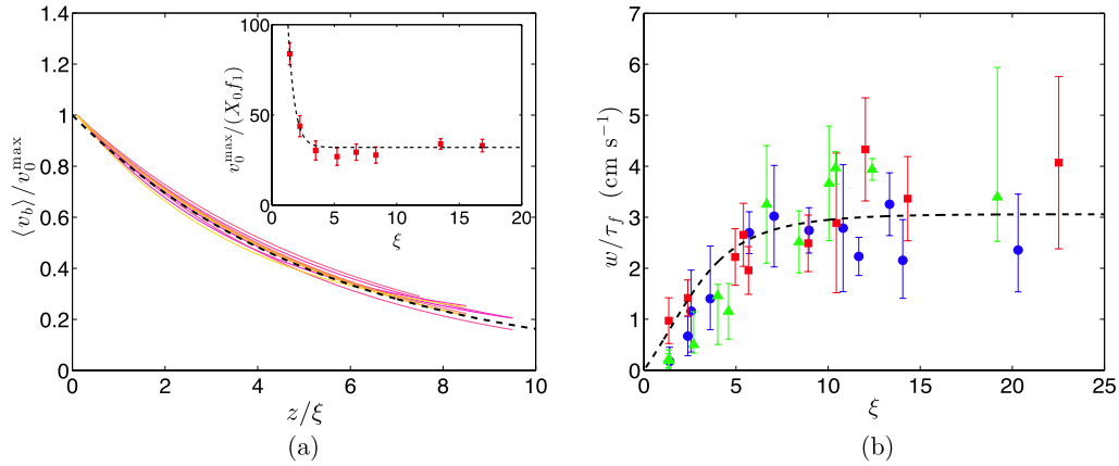
FIG. 6. (a) Velocity of the bubbles v_b averaged over one period and normalized by v_0^{max} = v_b(z/\xi = 0) as a function of the vertical position z/\xi in a foam made of 9 layers of bubbles. The curves correspond to different locations x and the black dotted line is the exponential fit \exp[-z/(5.2\xi)] . Inset: Evolution of the rescaled maximum value of the mean velocity of the bubbles v_0^{max}/(X_0 f_1) as a function of \xi . The dotted line corresponds to an exponential fit of the experimental measurements. These measurements are obtained in a w = 0.3 cm wide cell of length L = 7 cm and a height of foaming solution H = 4 cm. (b) Rescaled damping coefficient w/\tau_f as a function of \xi for various widths of the cell: w = 0.3 cm (blue circles), w = 0.6 cm (green triangles), and w = 1.6 cm (red squares) in L = 7 cm cells. The black dashed line shows the best fit adjusting the prefactor in the Eq. (14).
