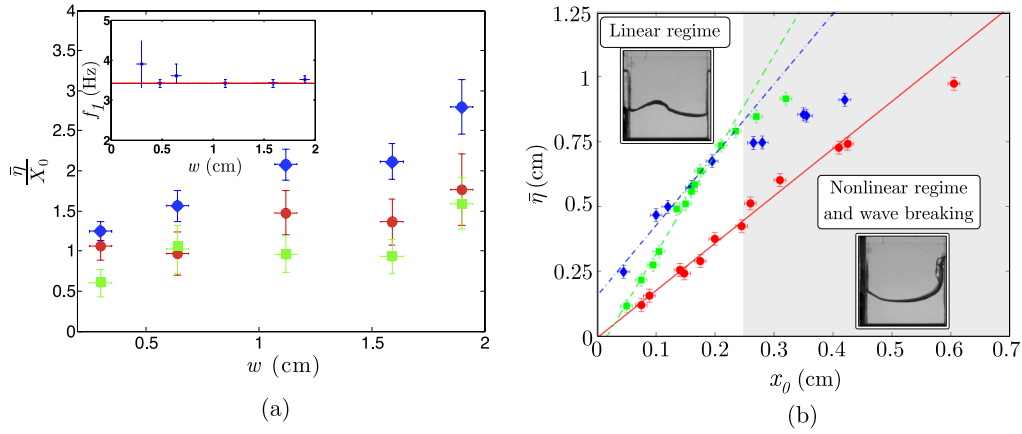
FIG. 8. (a) Rescaled maximum amplitude \bar{\eta}/X_0 averaged over x as a function of the width of the cell w for a forcing frequency f = 4 Hz (blue diamonds), f = 5 Hz (red circles), and f = 7 Hz (green squares). Inset: evolution of the first resonant frequency f_1 as a function of w . (b) Maximum amplitude of sloshing \bar{\eta} averaged over x as a function of the amplitude of the moving stage X_0 for a frequency f = 3.1 Hz and a width w = 0.3 cm (green squares), a frequency f = 3.5 Hz and a width w = 1.6 cm (blue diamonds), and a frequency f = 4.8 Hz and a width w = 1.6 cm (red circles).
